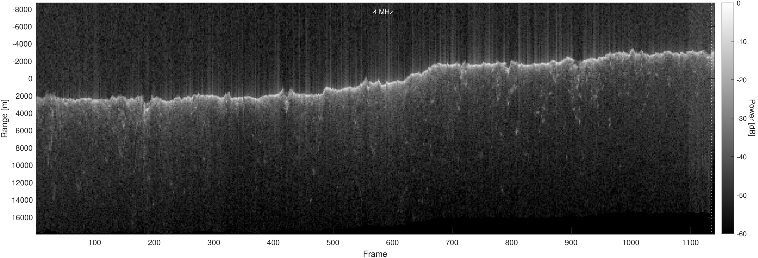
Orbit 17526, Optimized, No Window, Depth-Corrected, Channel 2
