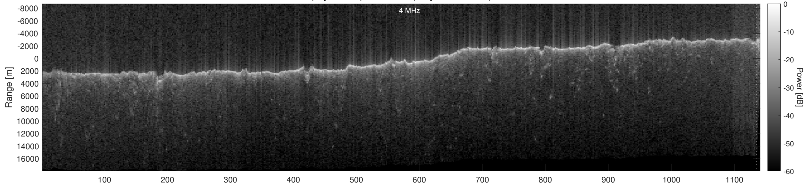
Orbit 17526, Optimized, No Window, Depth-Corrected, Channel 2
