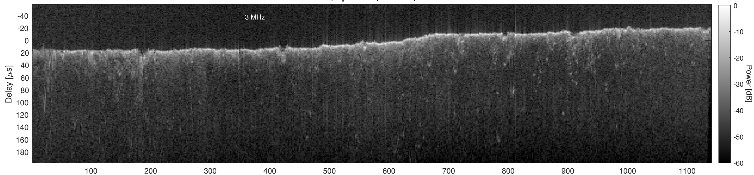
Orbit 17526, Cluttergram
