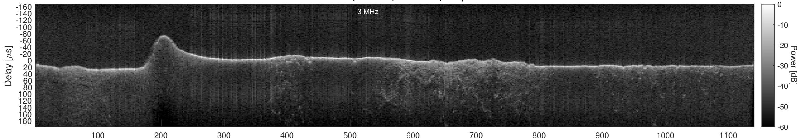
Orbit 17527, Window, Channel 2, Optimized
