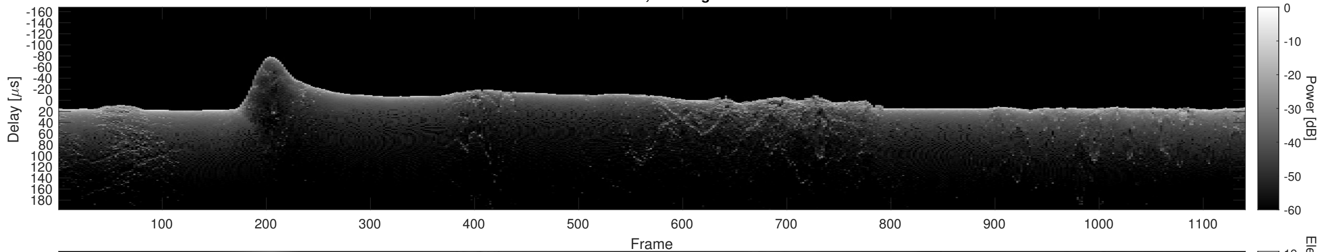
Orbit 17527, Cluttergram
