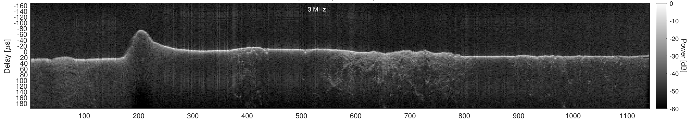
Orbit 17527, Window, Channel 2, Chapman
