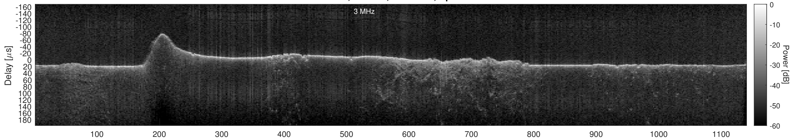
Orbit 17527, Cluttergram
