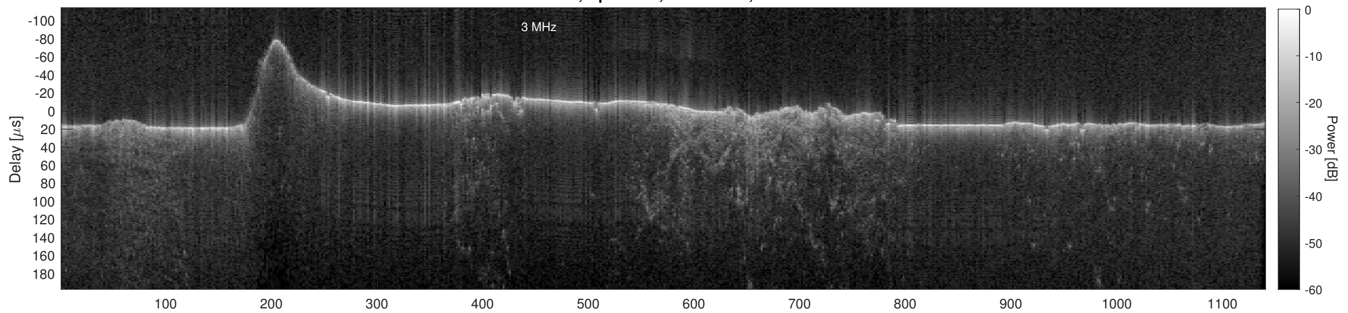
Orbit 17527, Cluttergram
