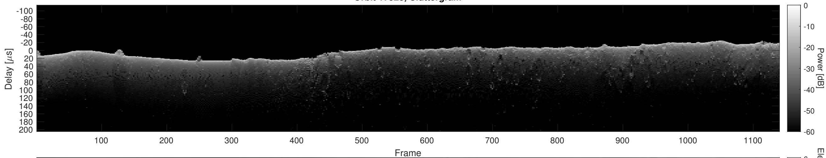
Orbit 17528, Cluttergram
