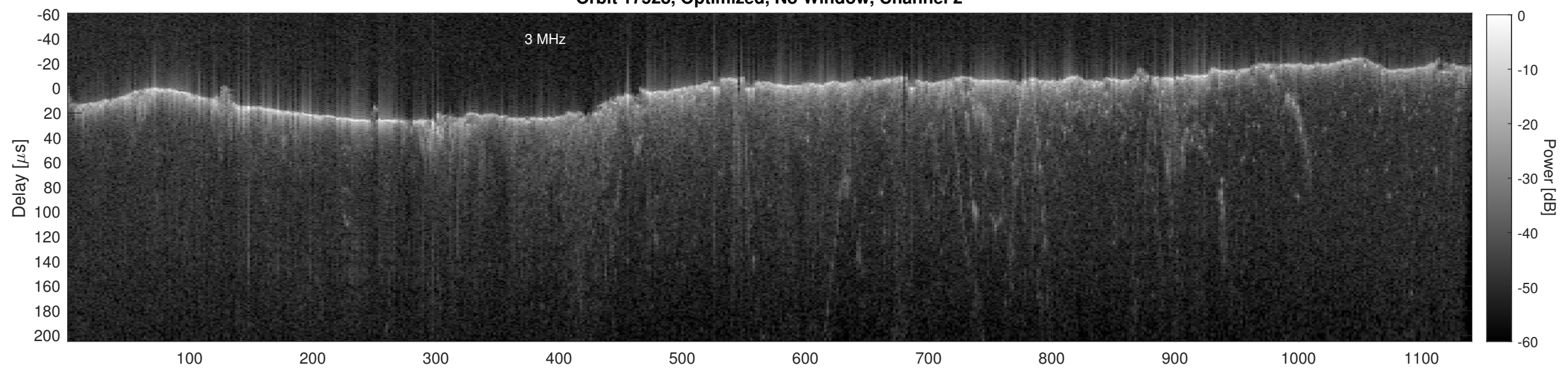
Orbit 17528, Cluttergram
