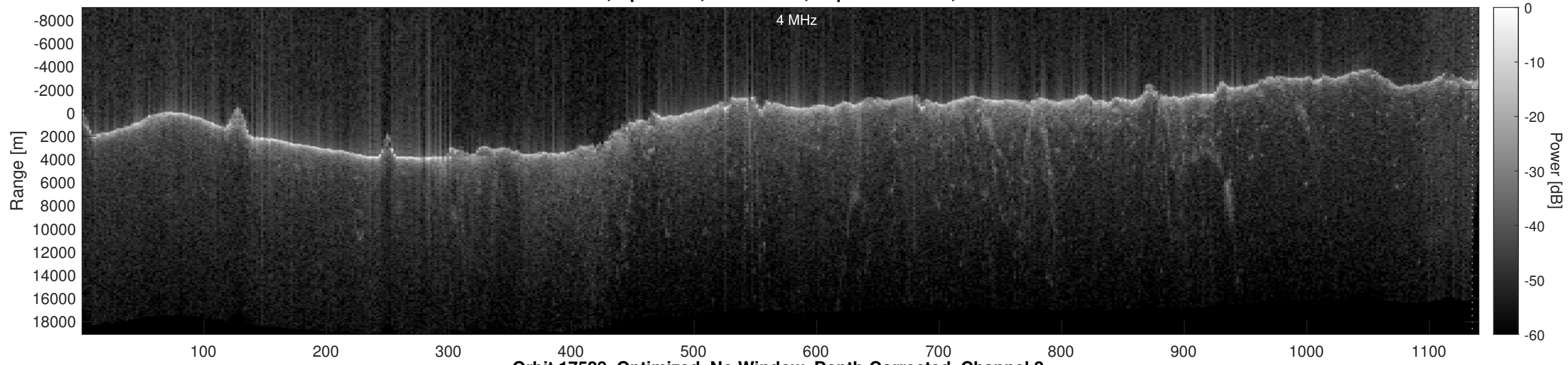
Orbit 17528, Optimized, No Window, Depth-Corrected, Channel 2
