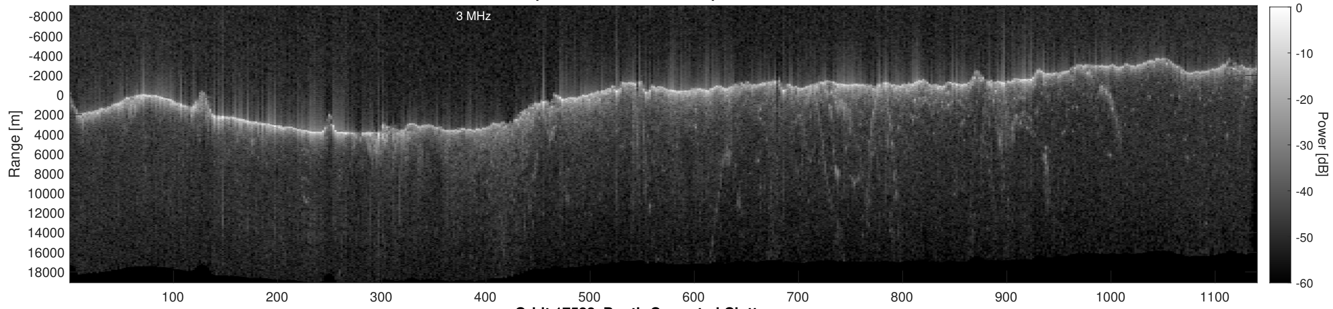
Orbit 17528, Depth-Corrected Cluttergram
