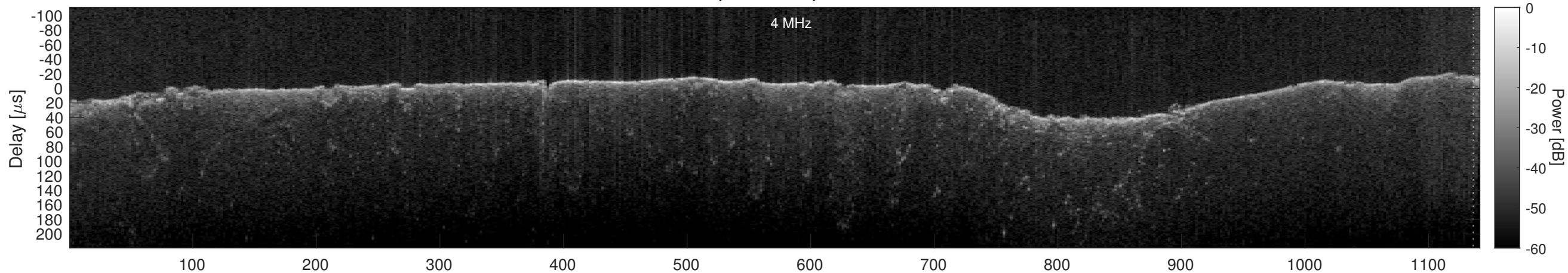
Orbit 17529, Window, Channel 1, Chapman
