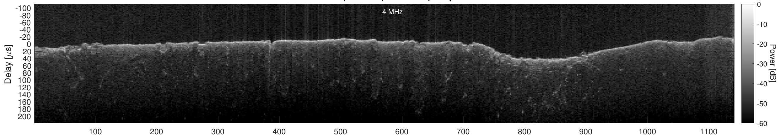
Orbit 17529, Window, Channel 1, Optimized
