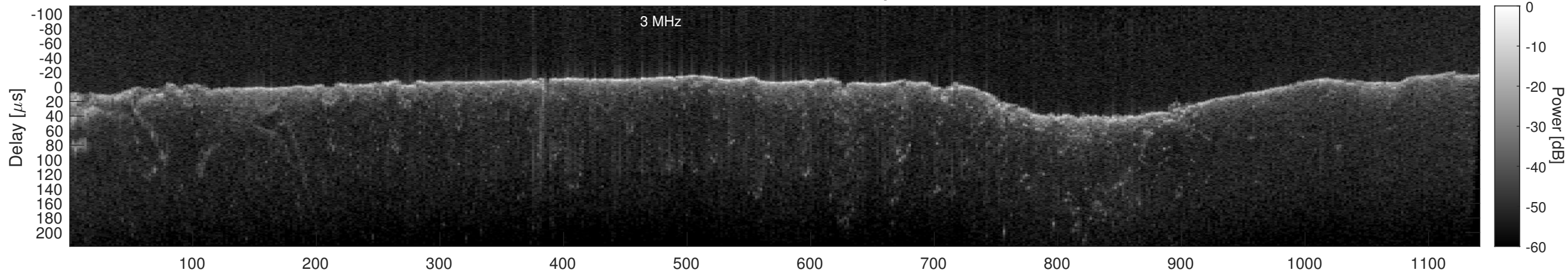
Orbit 17529, Cluttergram
