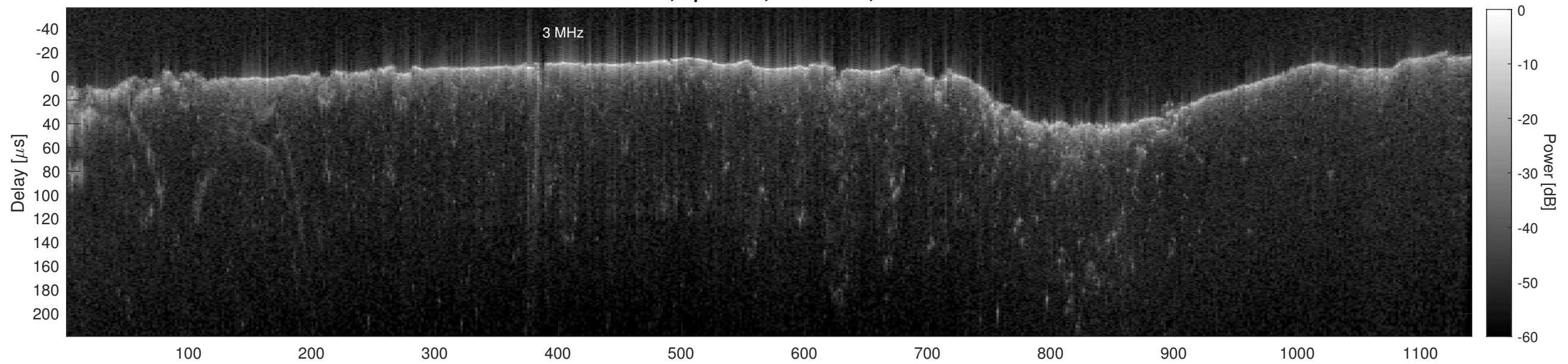
Orbit 17529, Cluttergram
