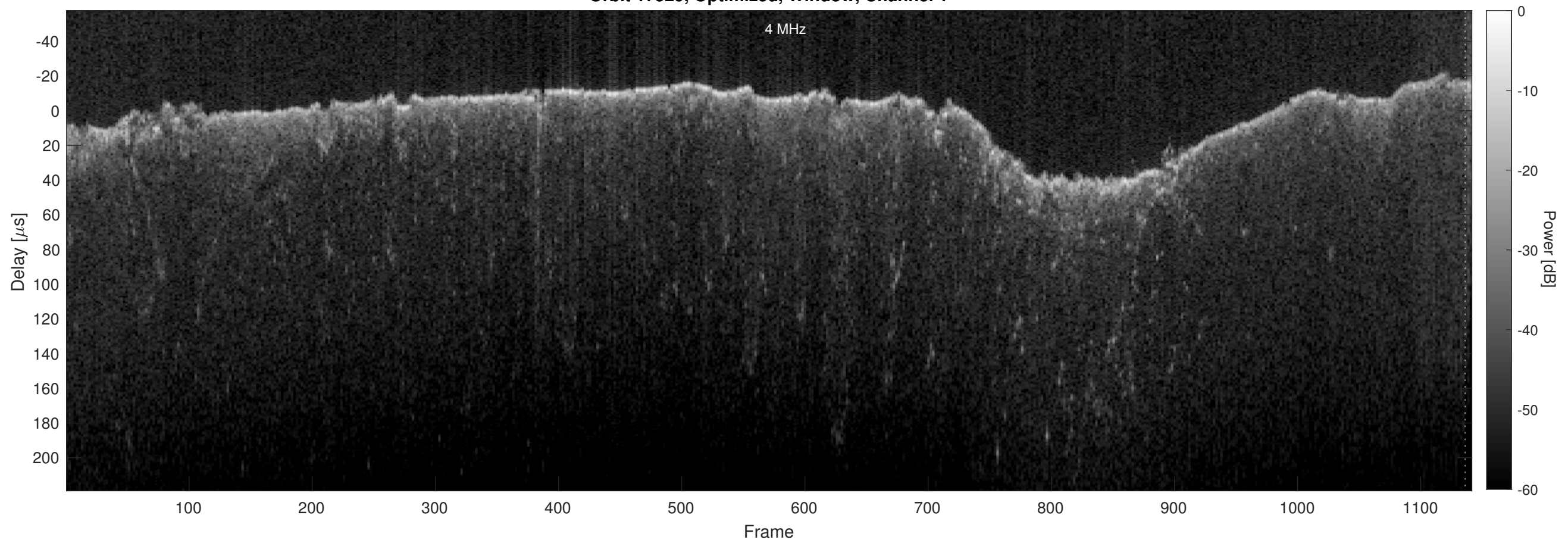
Orbit 17529, Optimized, Window, Channel 2
