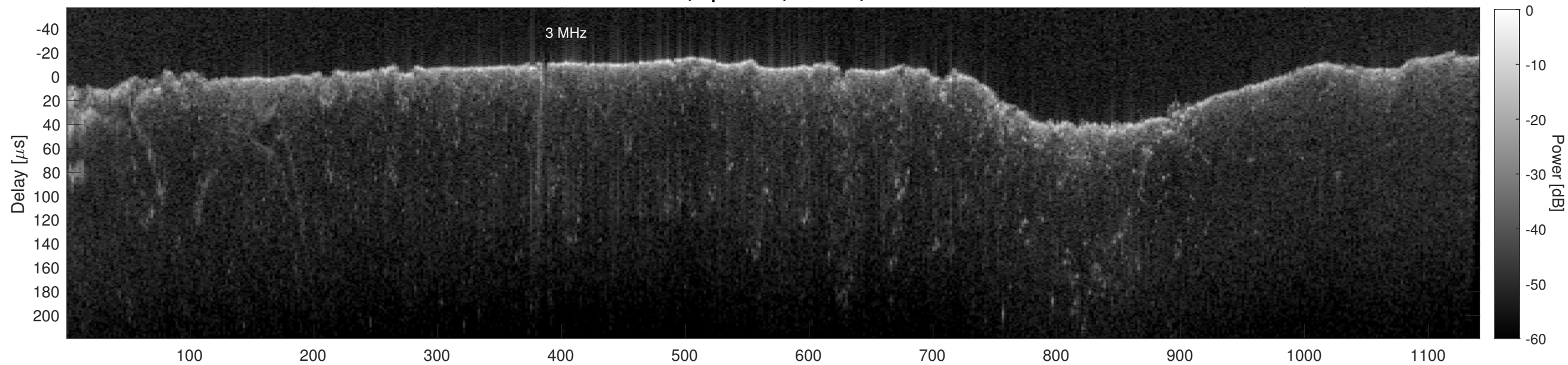
Orbit 17529, Cluttergram
