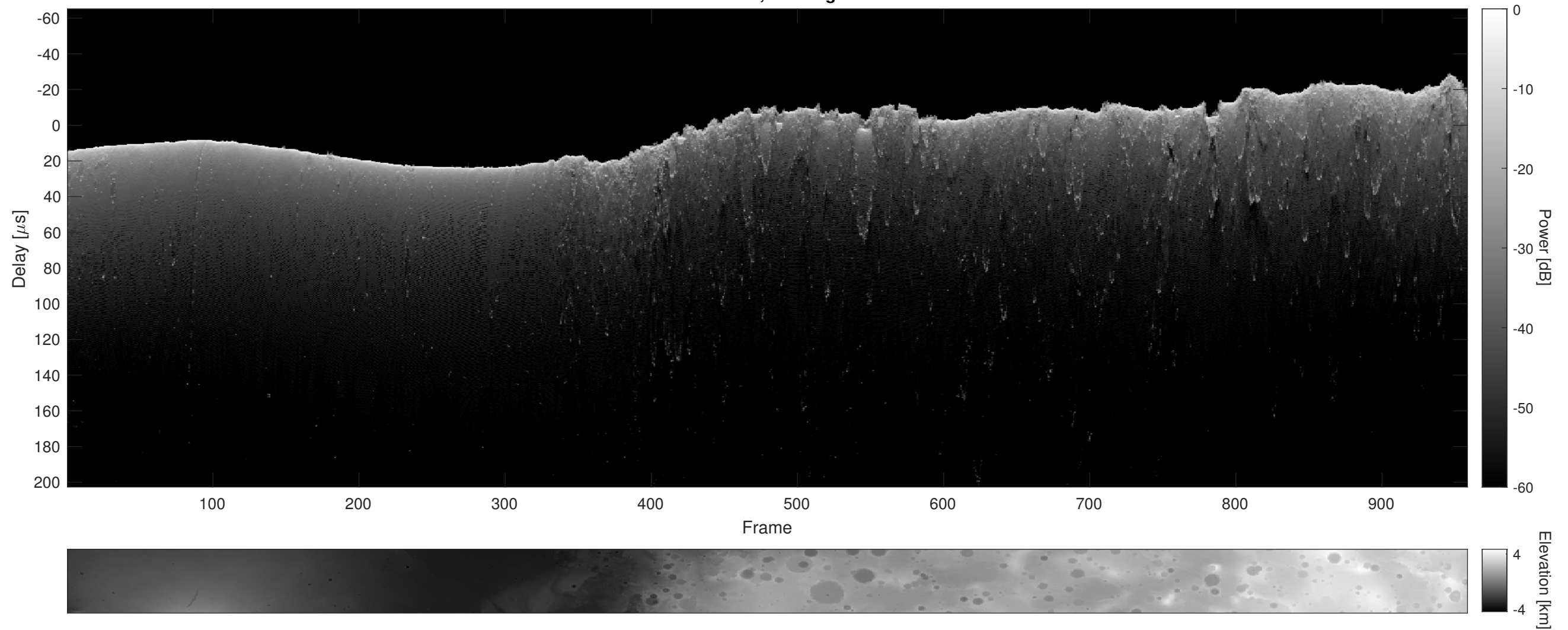
Orbit 17535, Cluttergram
