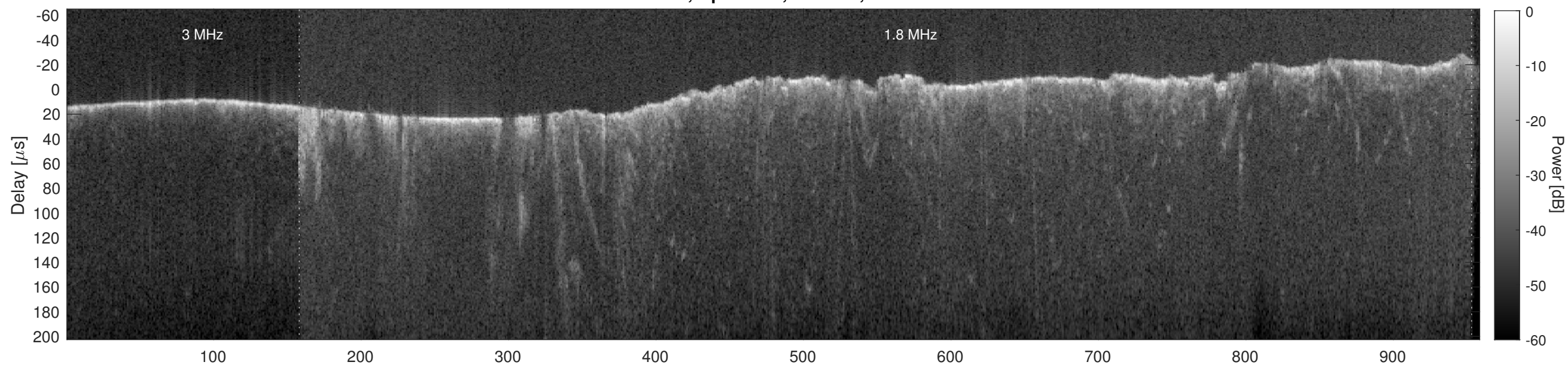
Orbit 17535, Cluttergram
