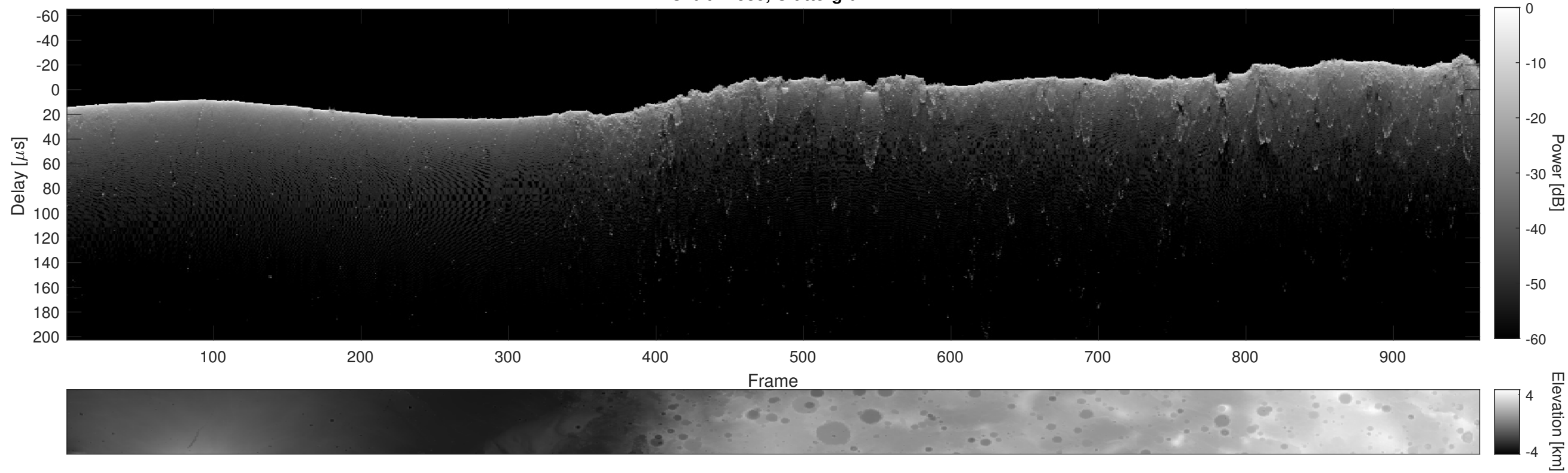
Orbit 17535, Cluttergram
