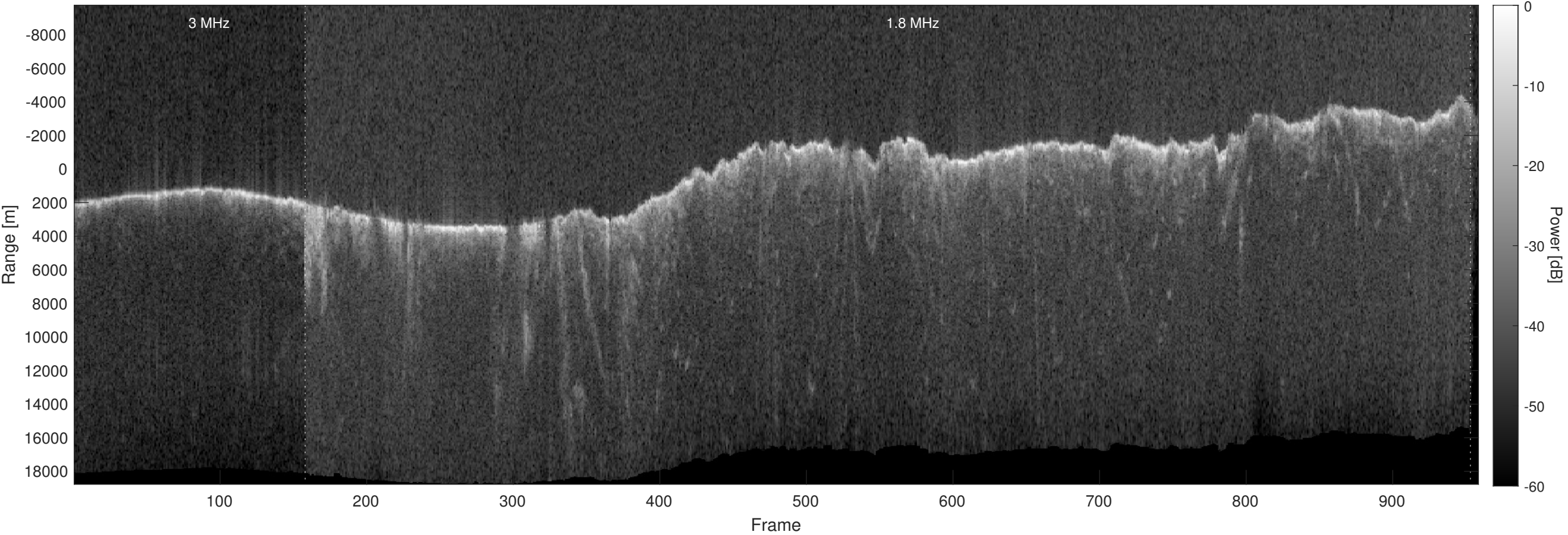
Orbit 17535, Optimized, Window, Depth-Corrected, Channel 2
