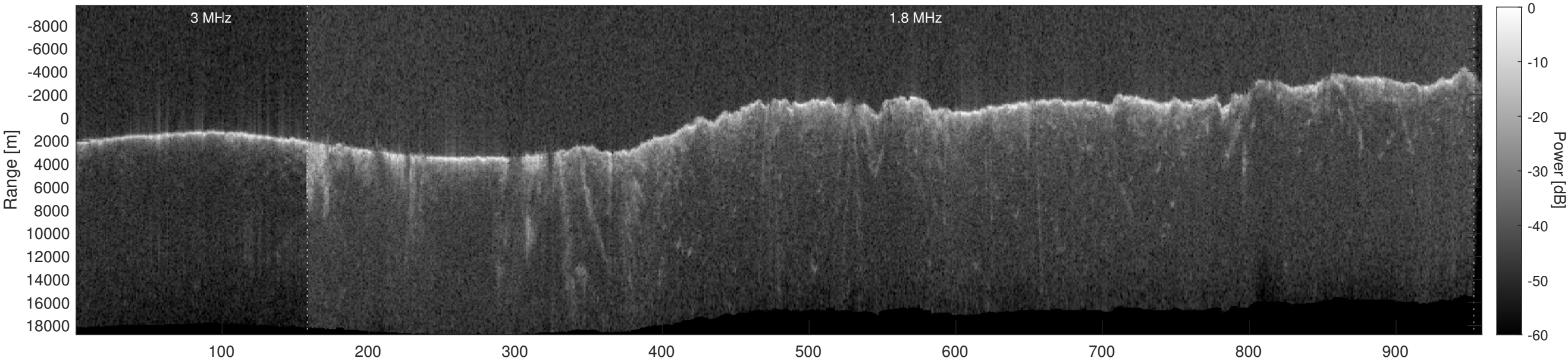
Orbit 17535, Depth-Corrected Cluttergram
