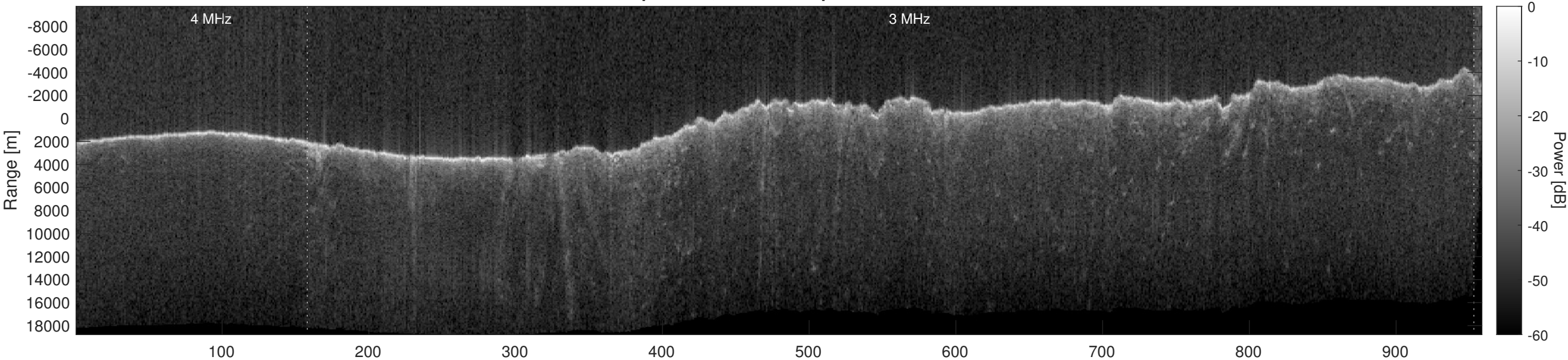
Orbit 17535, Optimized, Window, Depth-Corrected, Channel 2
