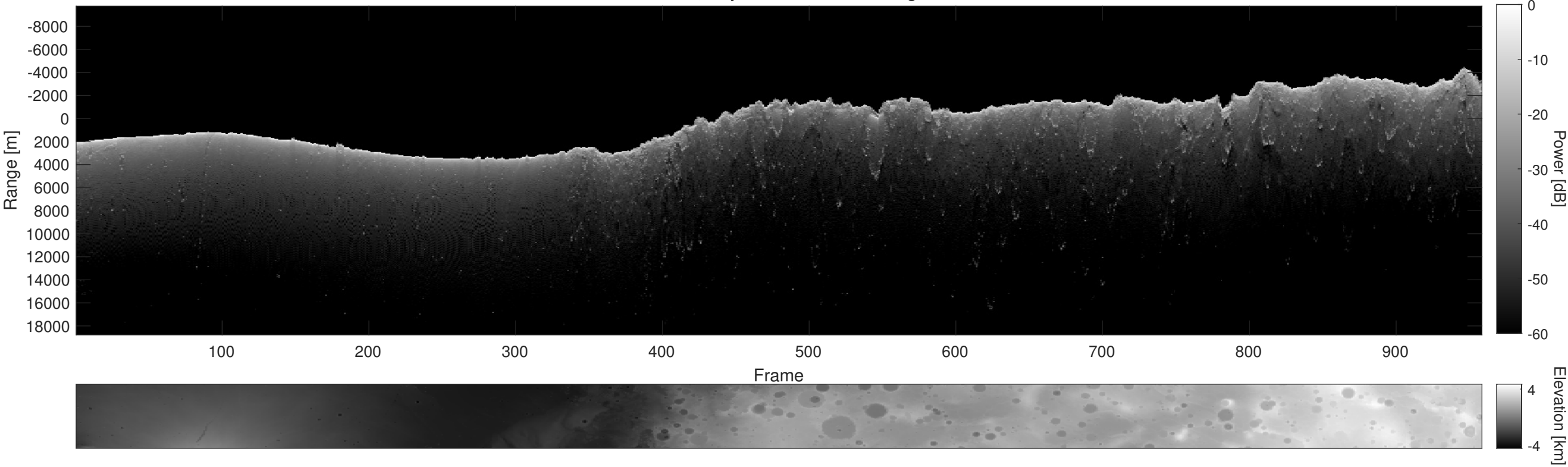
Orbit 17535, Depth-Corrected Cluttergram
