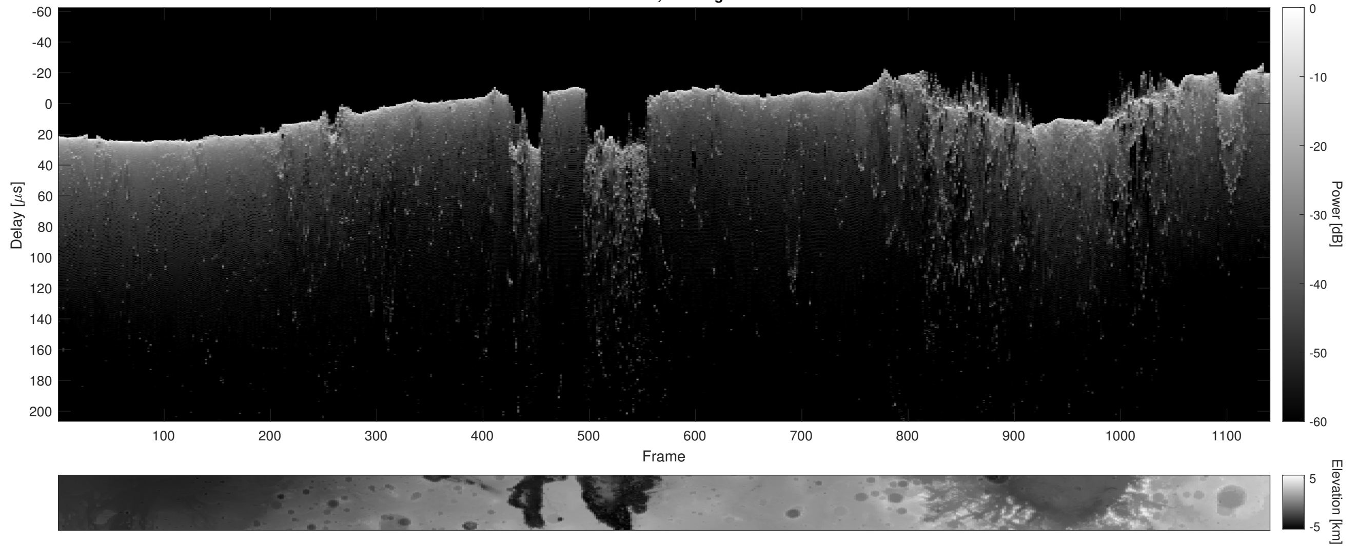
Orbit 17537, Cluttergram
