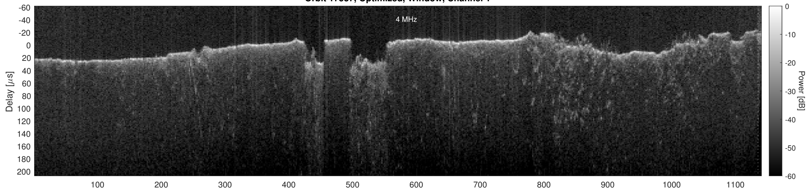
Orbit 17537, Optimized, Window, Channel 2
