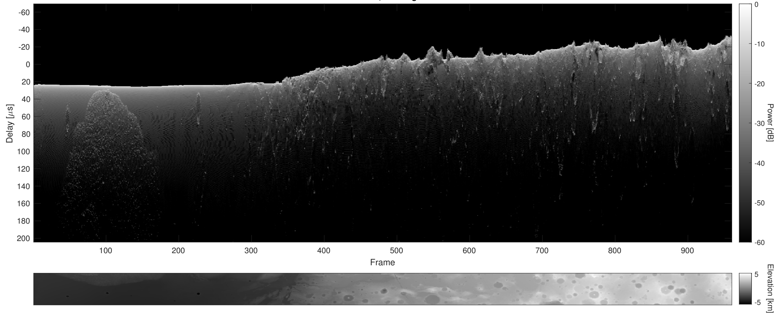
Orbit 17538, Cluttergram
