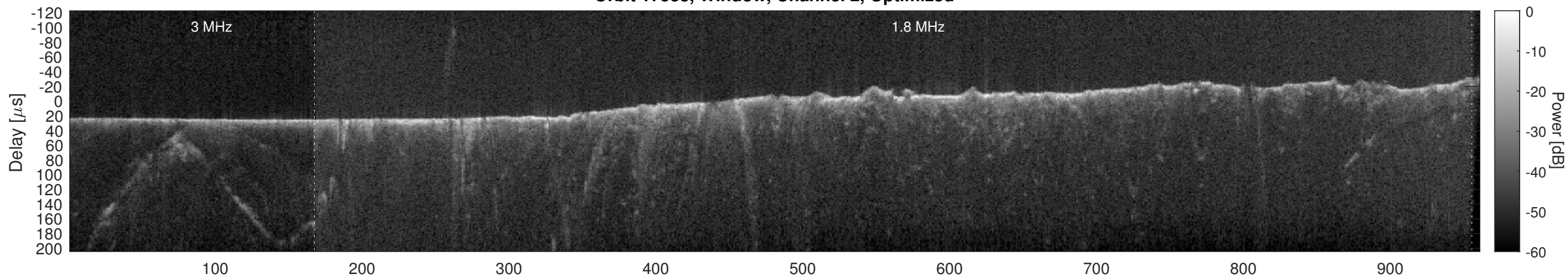
Orbit 17538, Cluttergram
