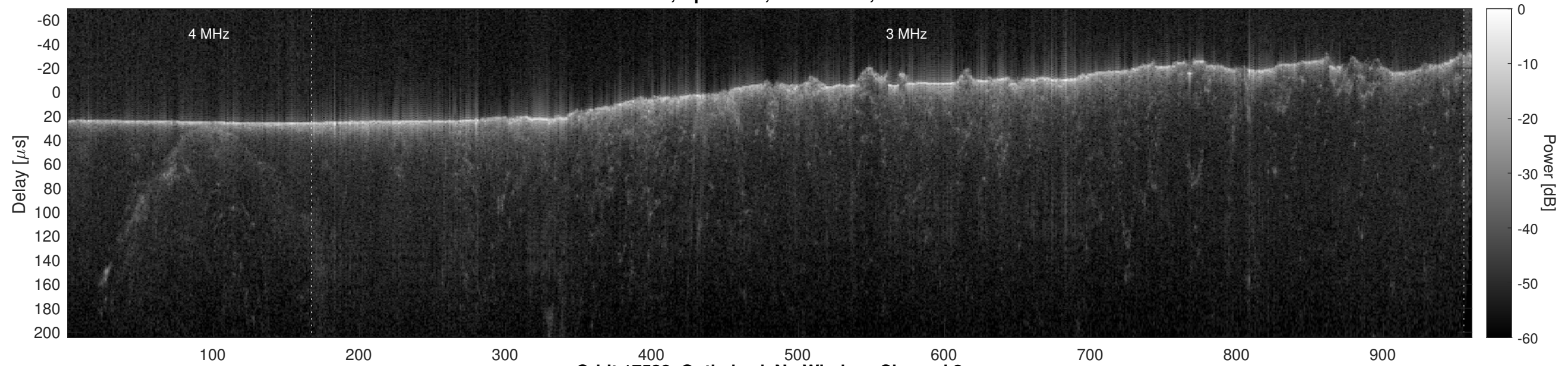
Orbit 17538, Optimized, No Window, Channel 2
