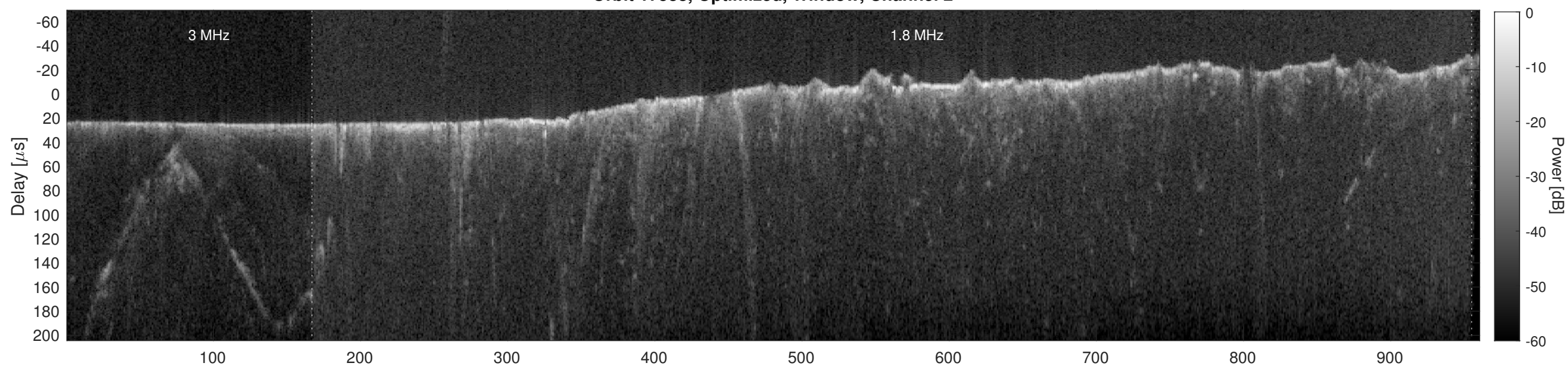
Orbit 17538, Cluttergram
