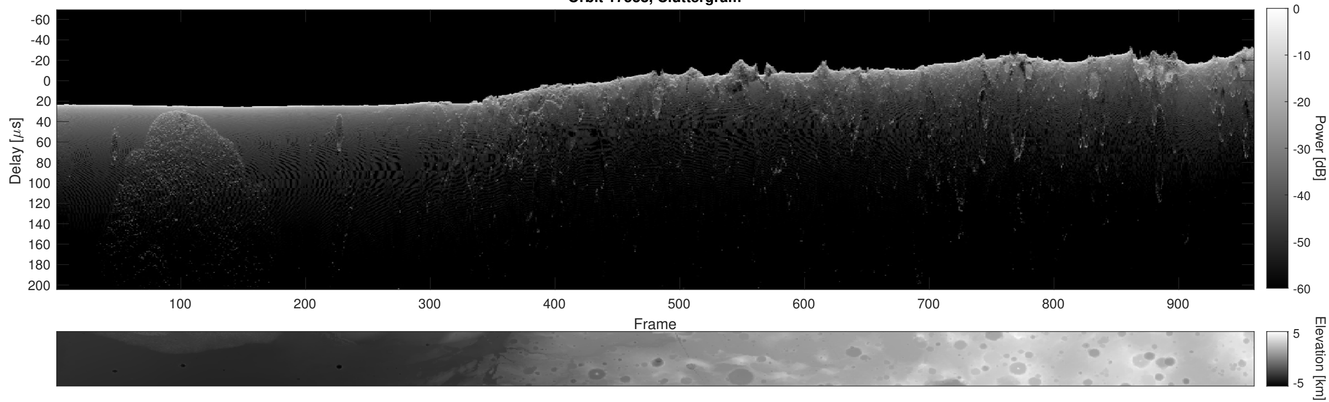
Orbit 17538, Cluttergram
