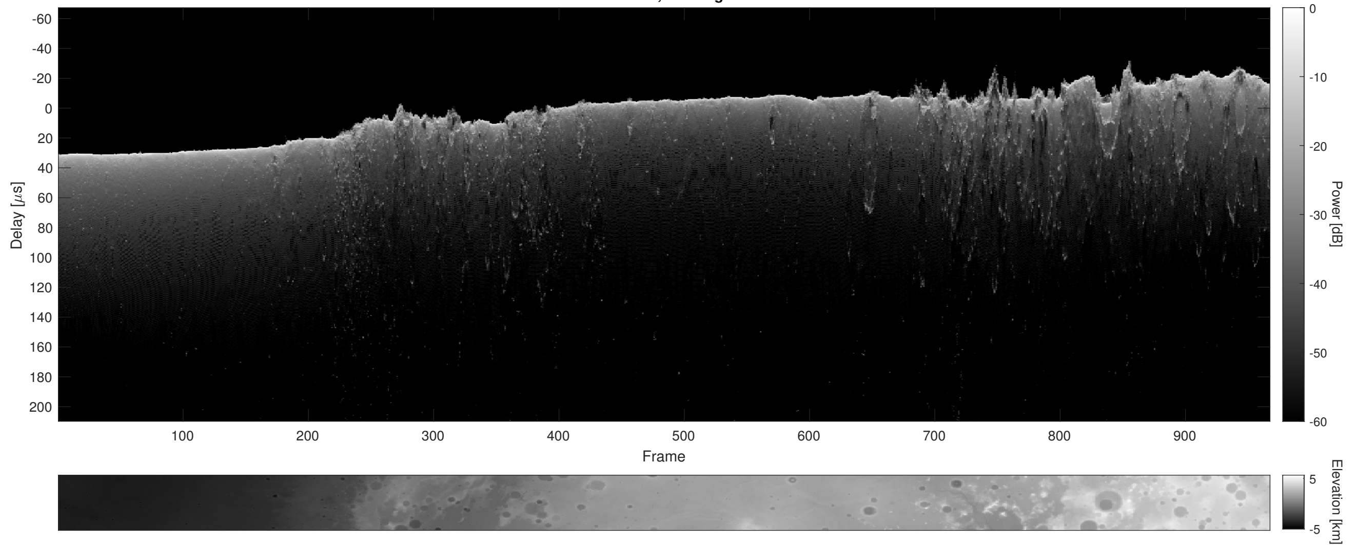
Orbit 17546, Cluttergram
