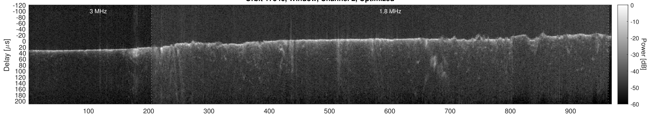
Orbit 17546, Cluttergram
