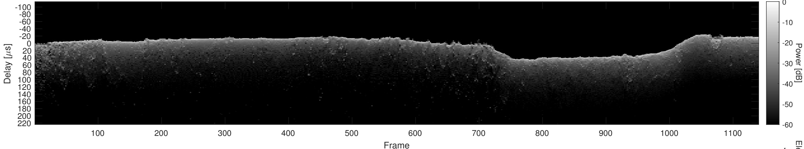
Orbit 17550, Cluttergram
