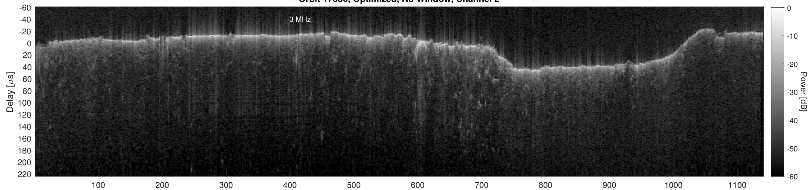
Orbit 17550, Cluttergram
