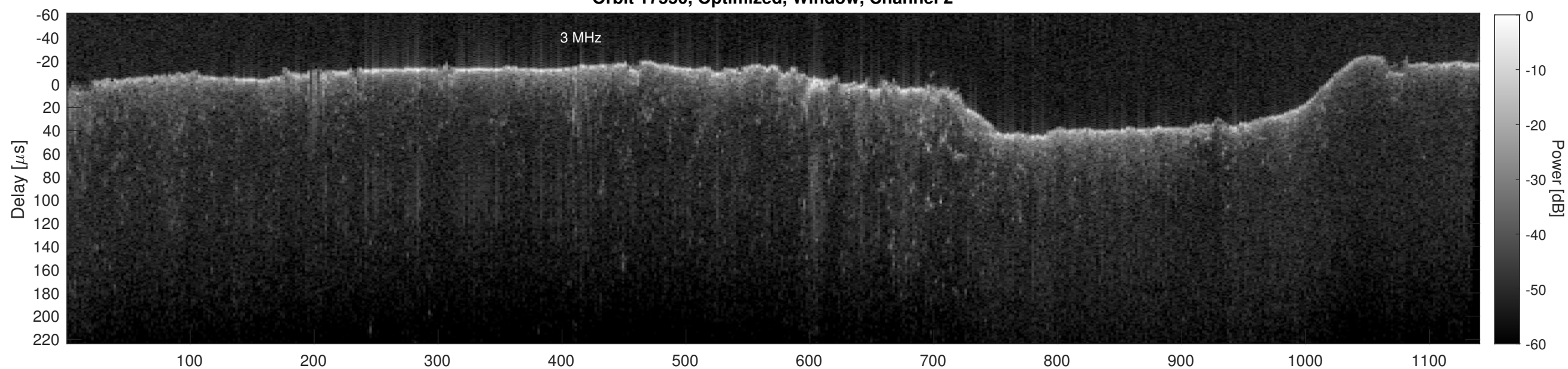
Orbit 17550, Cluttergram
