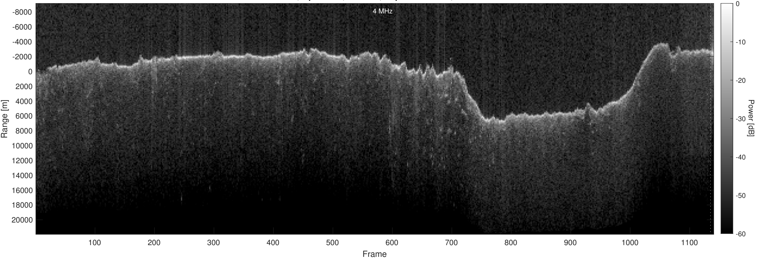
Orbit 17550, Optimized, Window, Depth-Corrected, Channel 2
