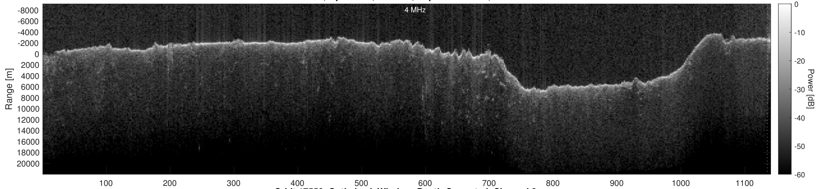
Orbit 17550, Optimized, Window, Depth-Corrected, Channel 2
