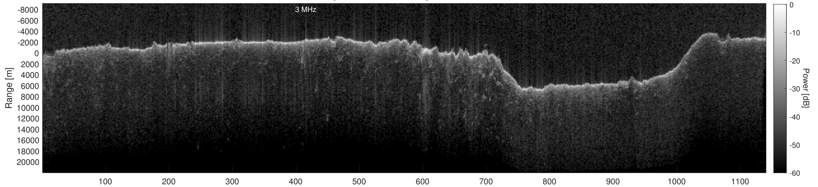
Orbit 17550, Depth-Corrected Cluttergram
