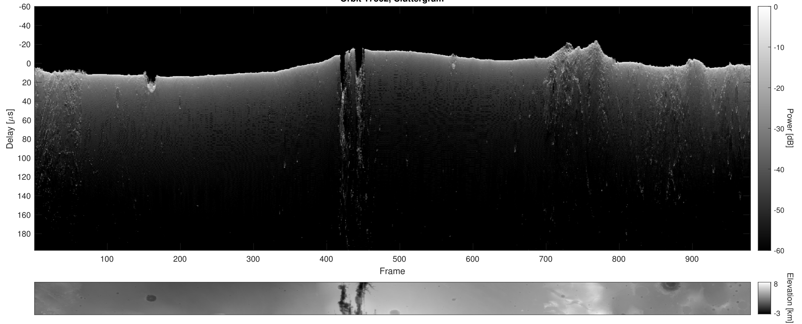
Orbit 17562, Cluttergram
