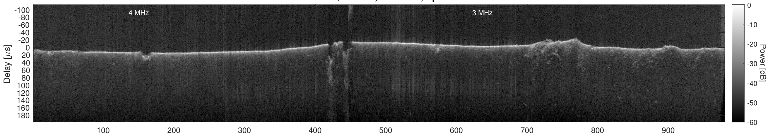
Orbit 17562, Cluttergram
