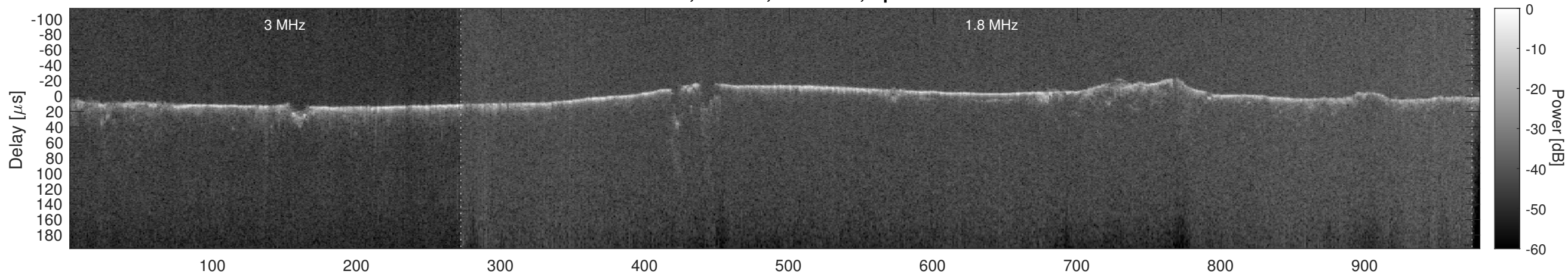
Orbit 17562, Cluttergram
