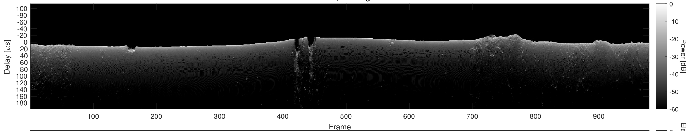
Orbit 17562, Cluttergram
