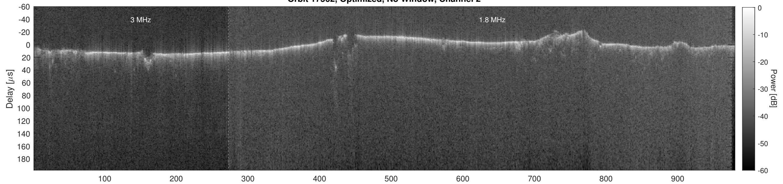
Orbit 17562, Cluttergram
