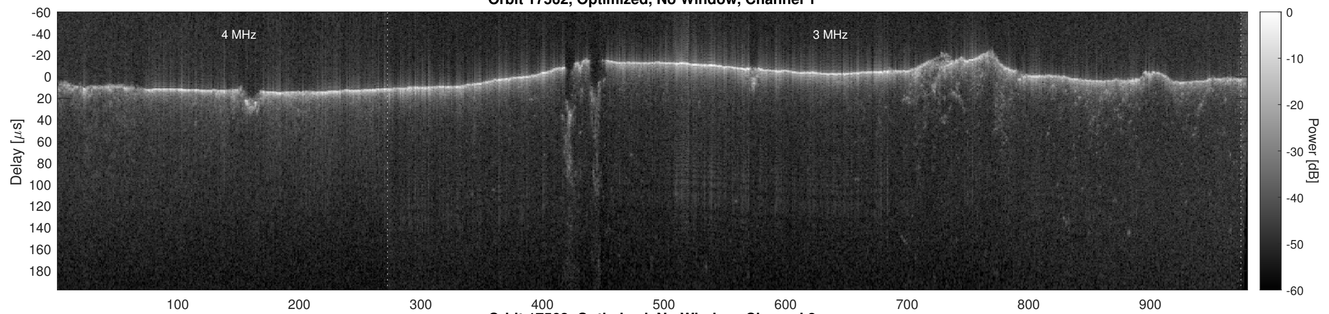
Orbit 17562, Optimized, No Window, Channel 2
