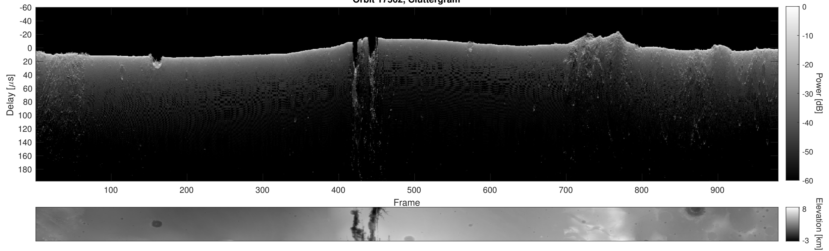
Orbit 17562, Cluttergram
