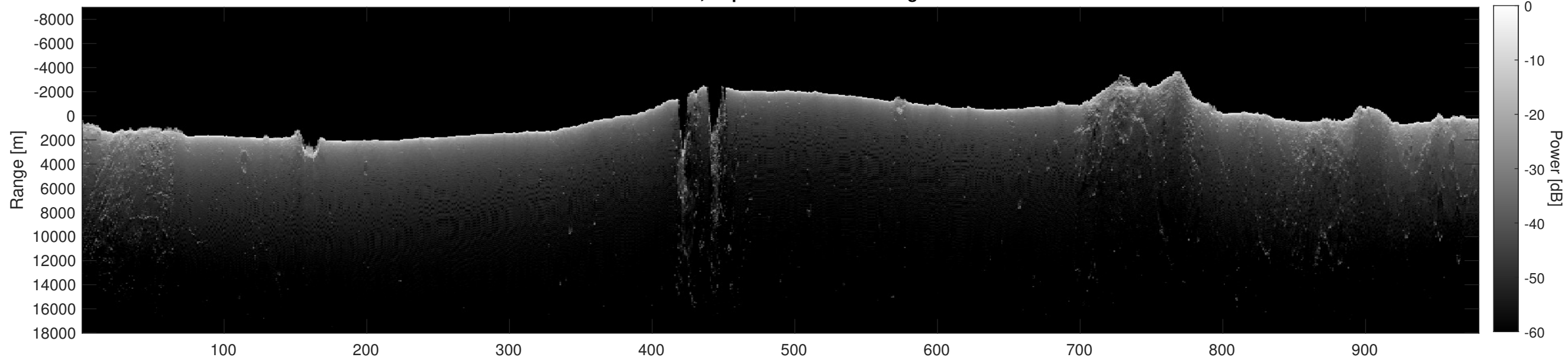
Orbit 17562, Depth-Corrected Cluttergram
