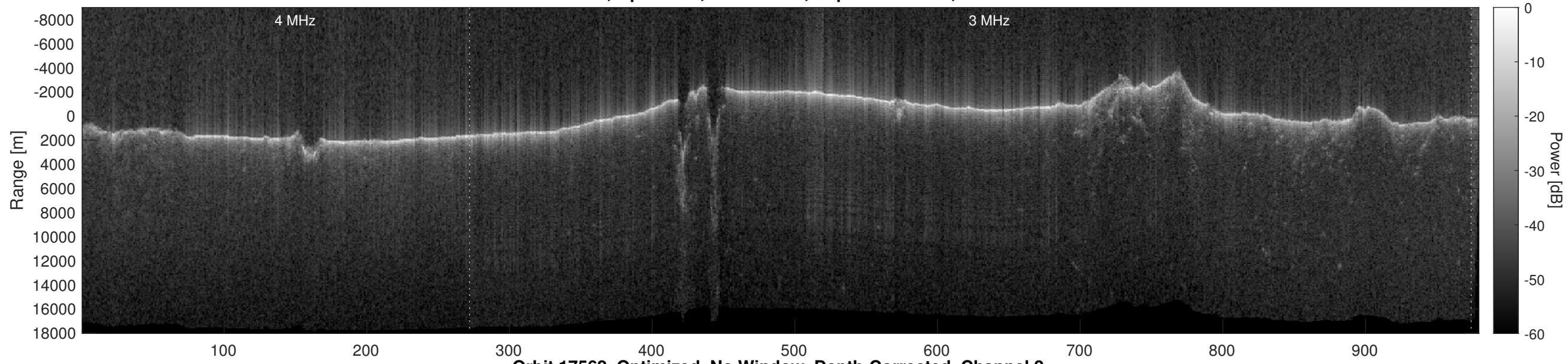
Orbit 17562, Optimized, No Window, Depth-Corrected, Channel 2
