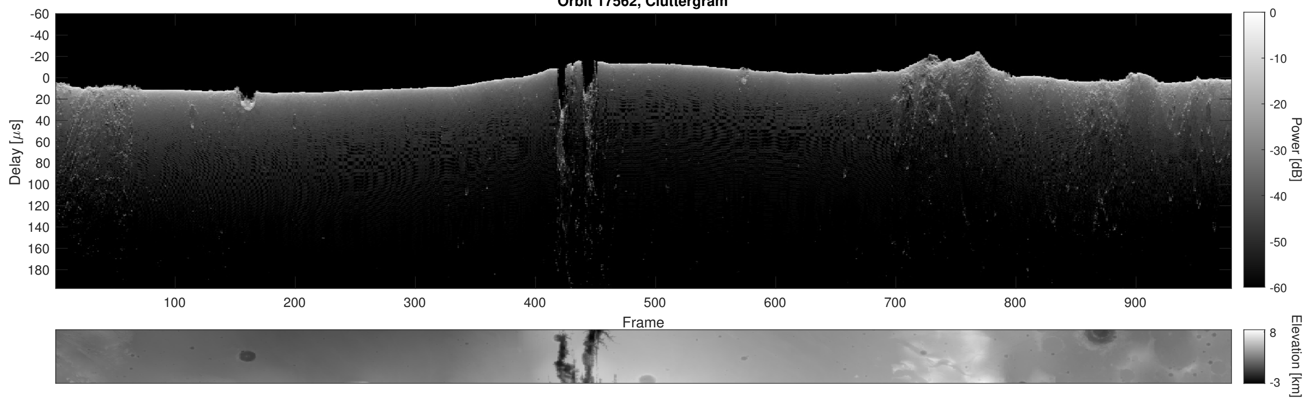
Orbit 17562, Cluttergram
