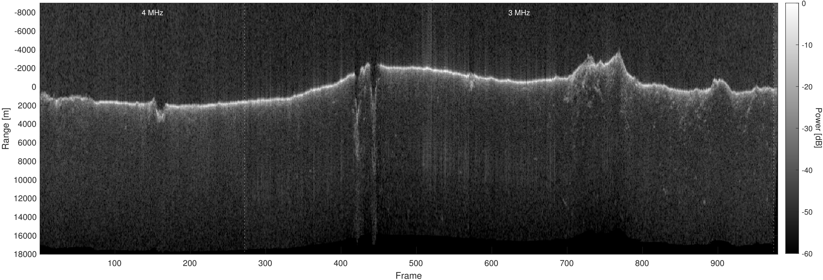
Orbit 17562, Optimized, Window, Depth-Corrected, Channel 2
