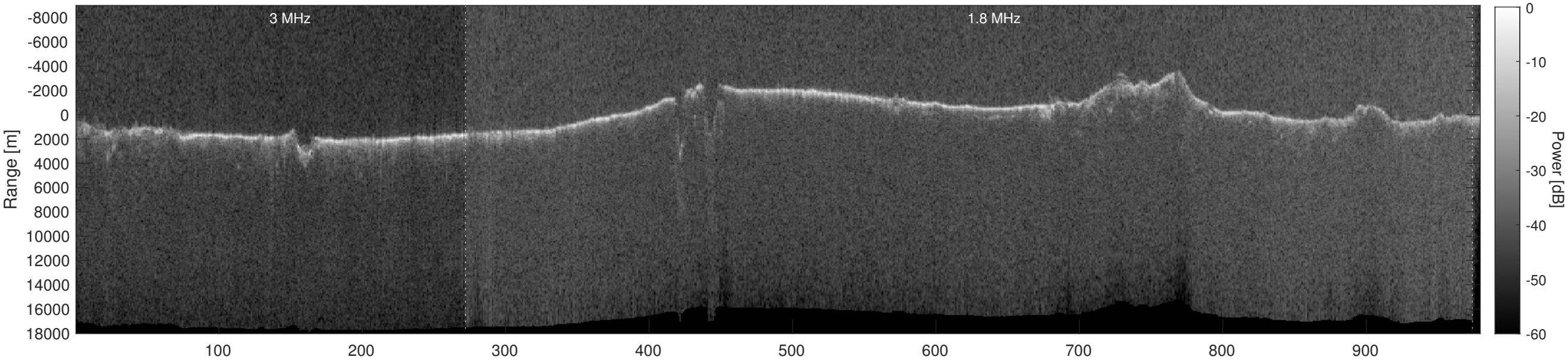
Orbit 17562, Depth-Corrected Cluttergram
