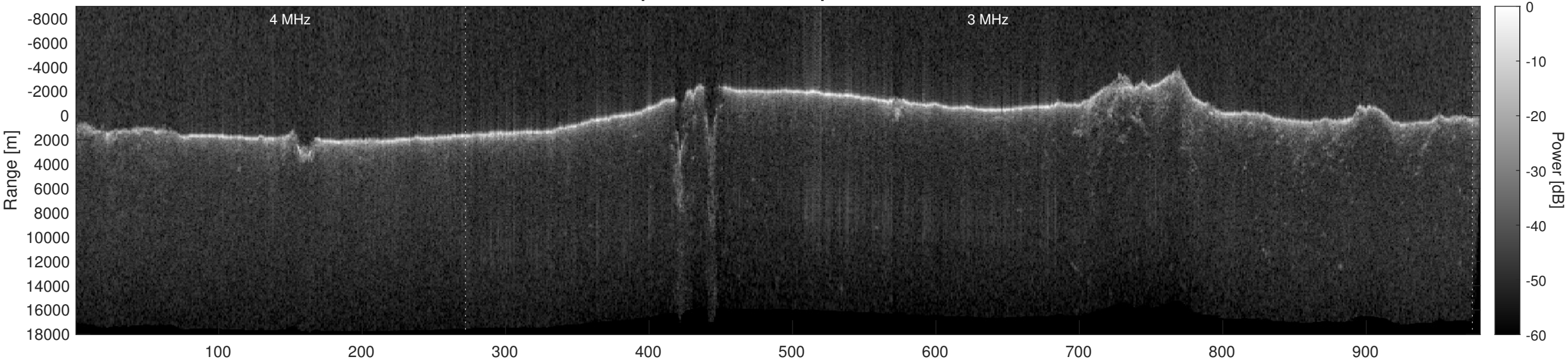
Orbit 17562, Optimized, Window, Depth-Corrected, Channel 2
