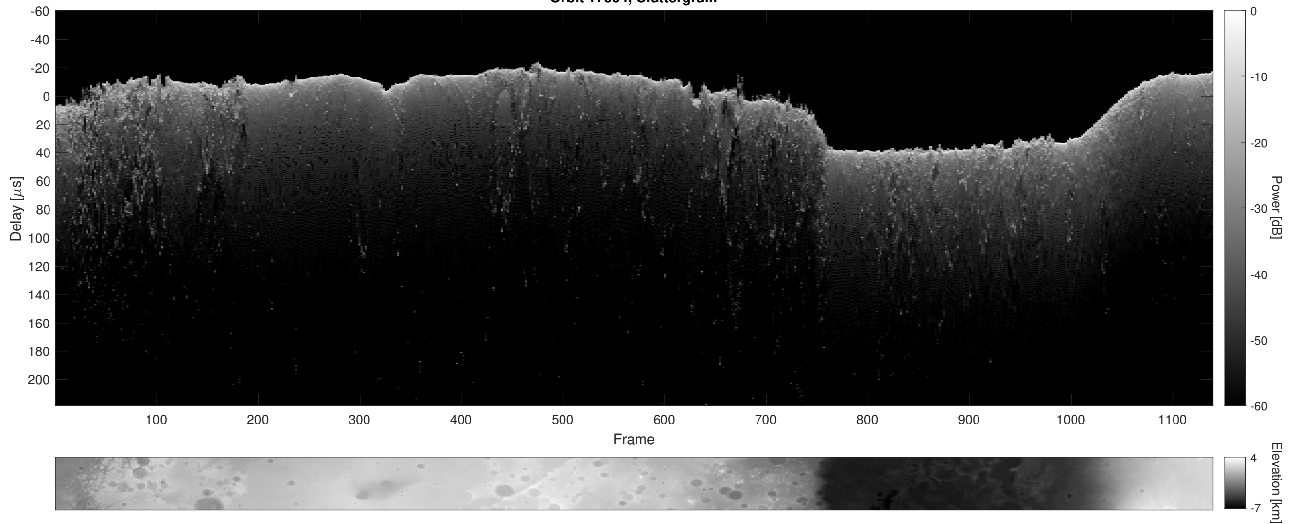
Orbit 17564, Cluttergram
