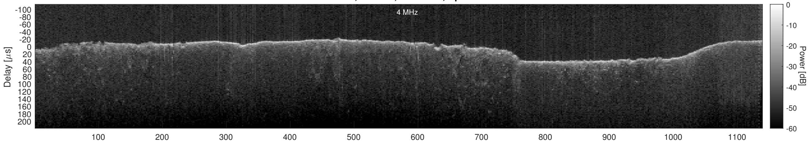
Orbit 17564, Cluttergram
