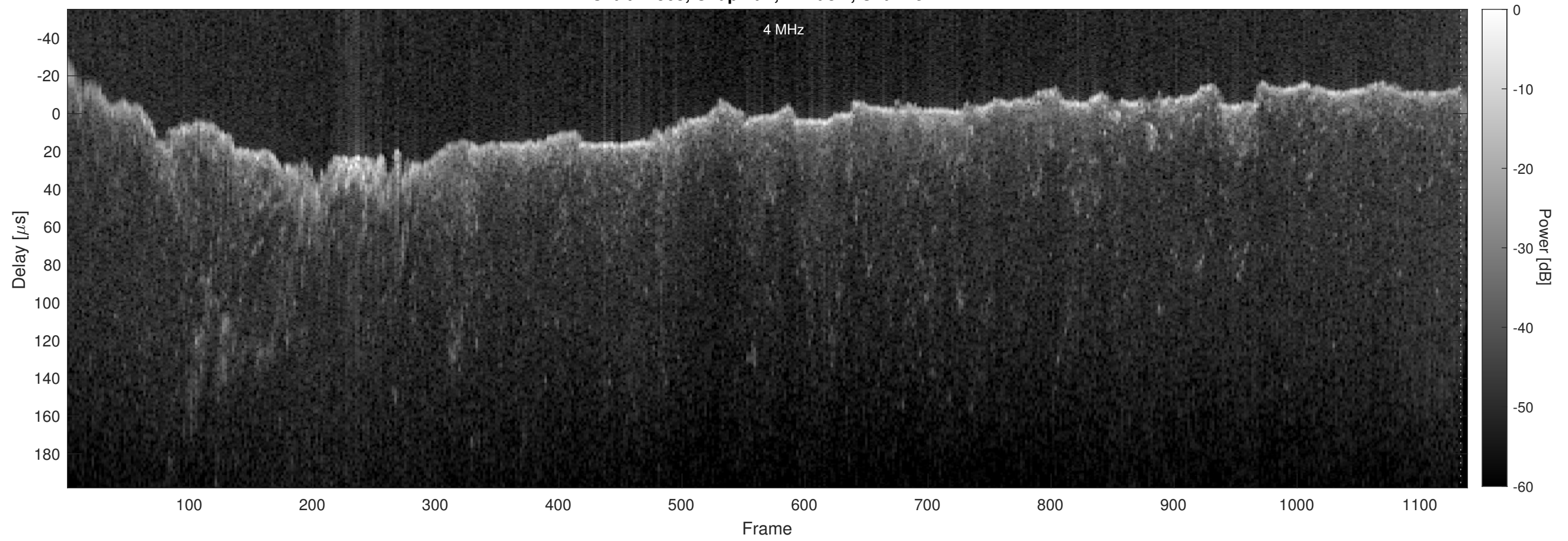
Orbit 17568, Chapman, Window, Channel 2
