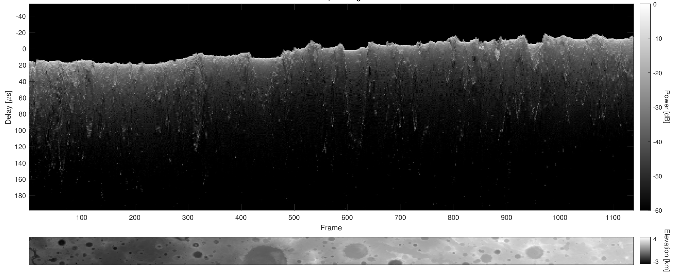
Orbit 17568, Cluttergram
