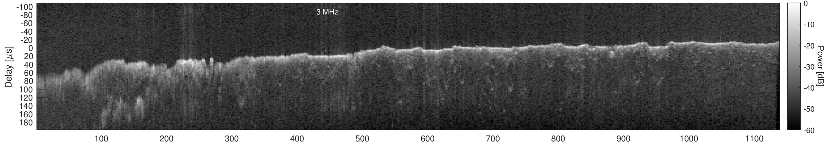
Orbit 17568, Window, Channel 2, Chapman
