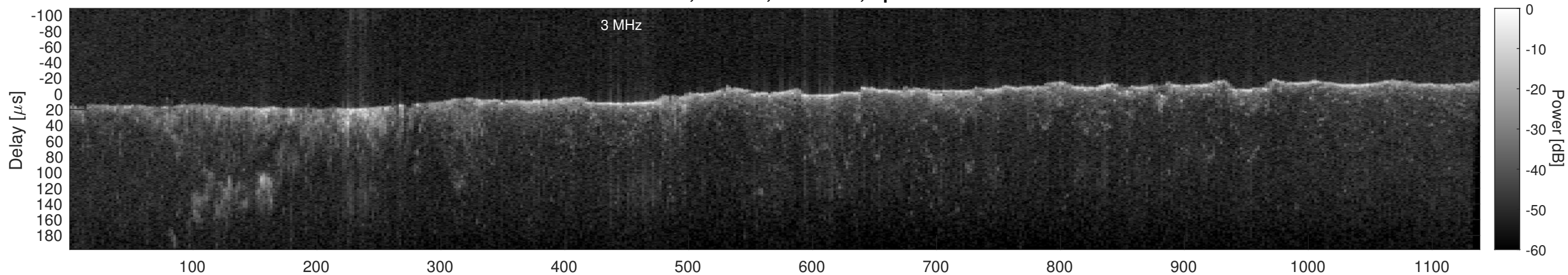
Orbit 17568, Cluttergram
