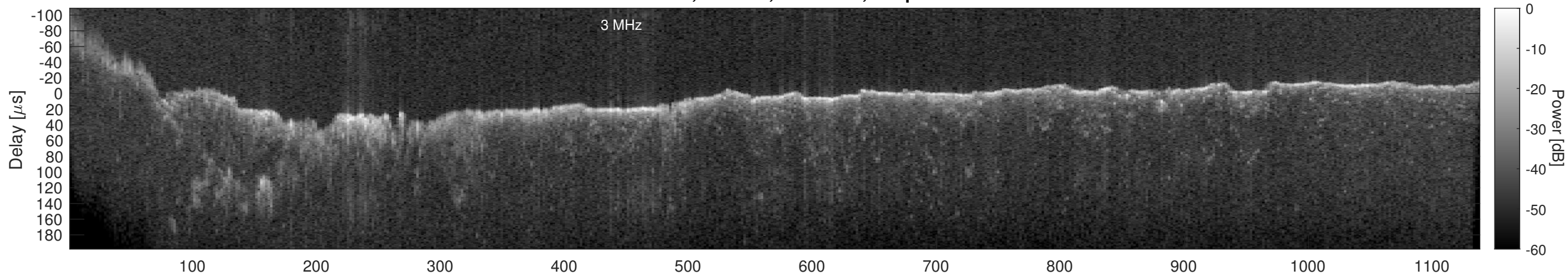
Orbit 17568, Window, Channel 2, Optimized
