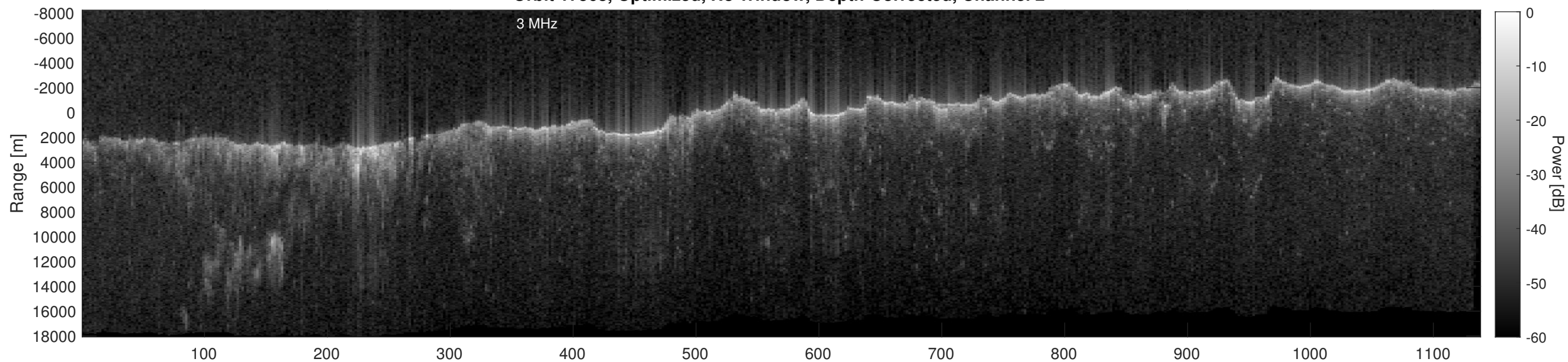
Orbit 17568, Depth-Corrected Cluttergram
