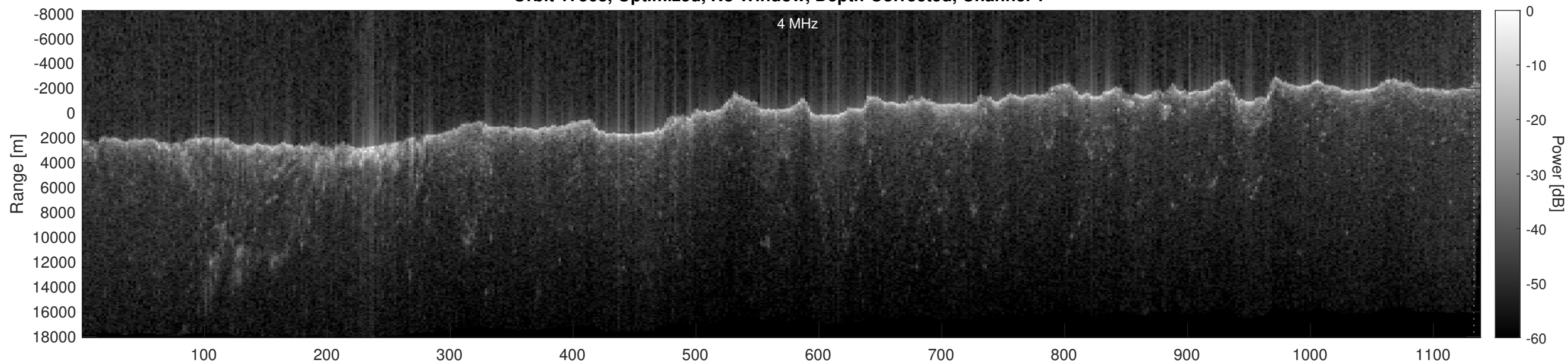
Orbit 17568, Optimized, No Window, Depth-Corrected, Channel 2
