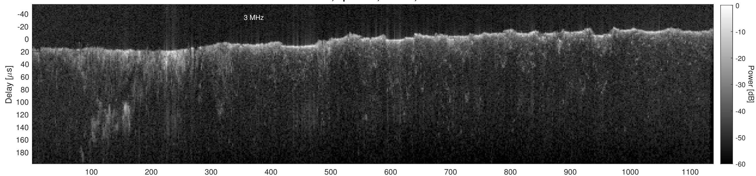
Orbit 17568, Cluttergram
