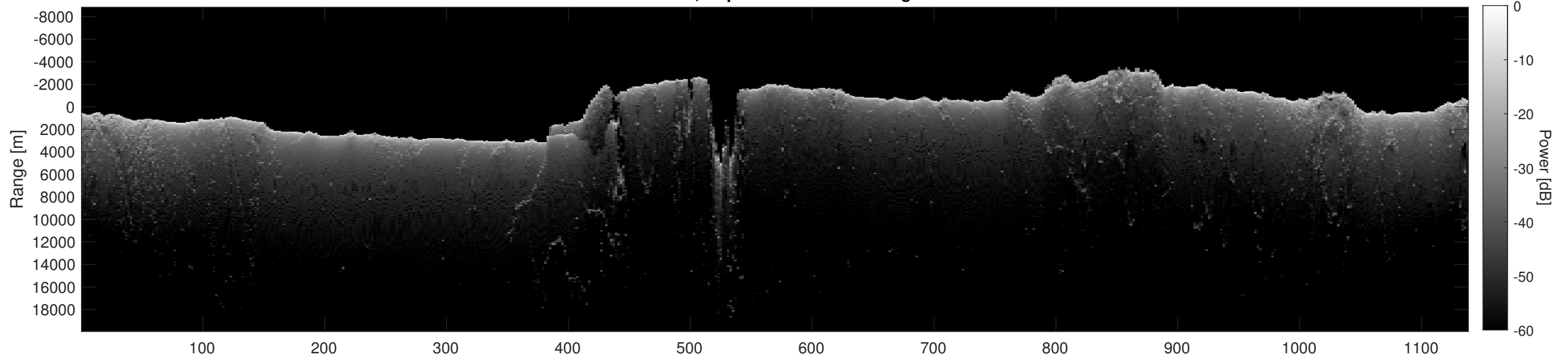
Orbit 17576, Depth-Corrected Cluttergram
