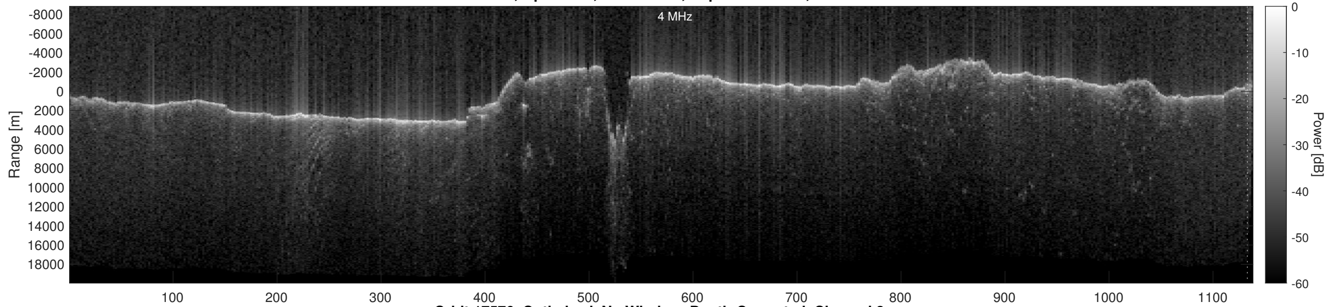
Orbit 17576, Optimized, No Window, Depth-Corrected, Channel 2
