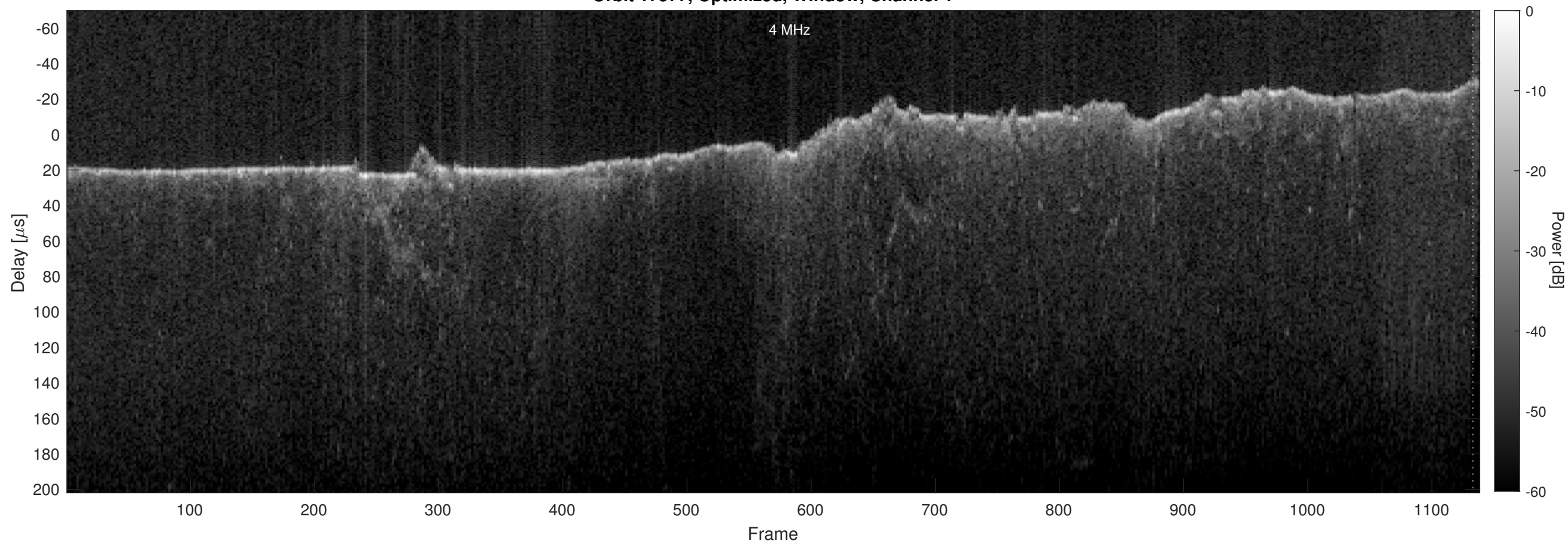
Orbit 17577, Optimized, Window, Channel 2
