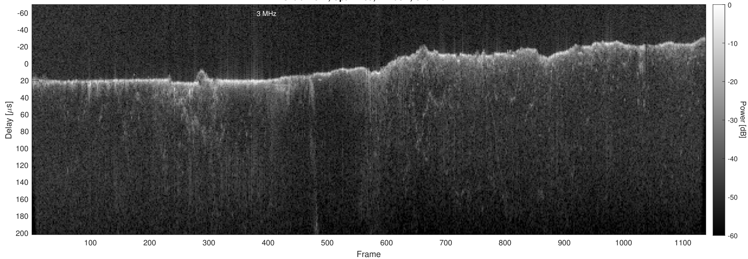
Orbit 17577, Optimized, Window, Channel 2
