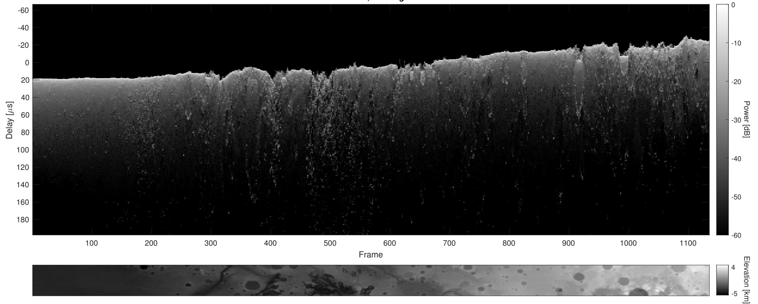
Orbit 17579, Cluttergram
