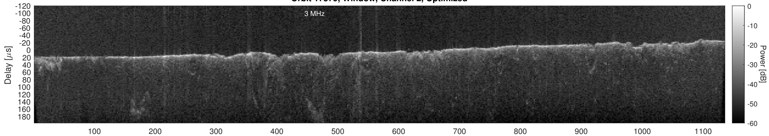
Orbit 17579, Cluttergram
