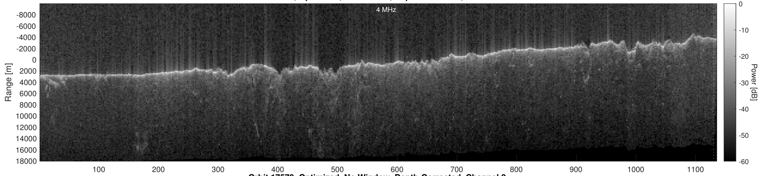
Orbit 17579, Optimized, No Window, Depth-Corrected, Channel 2
