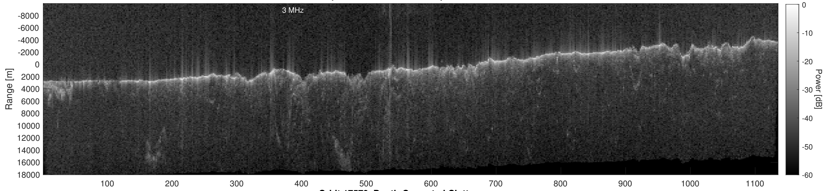
Orbit 17579, Depth-Corrected Cluttergram
